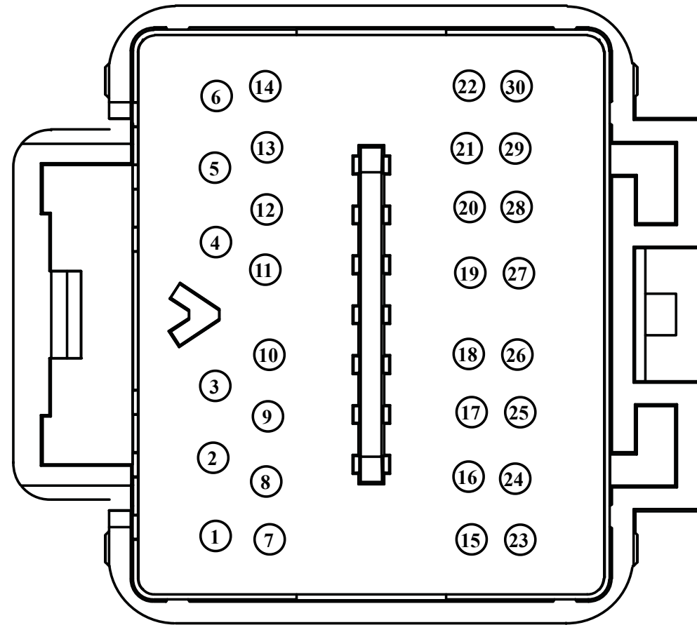
MALE Harness 14A005
