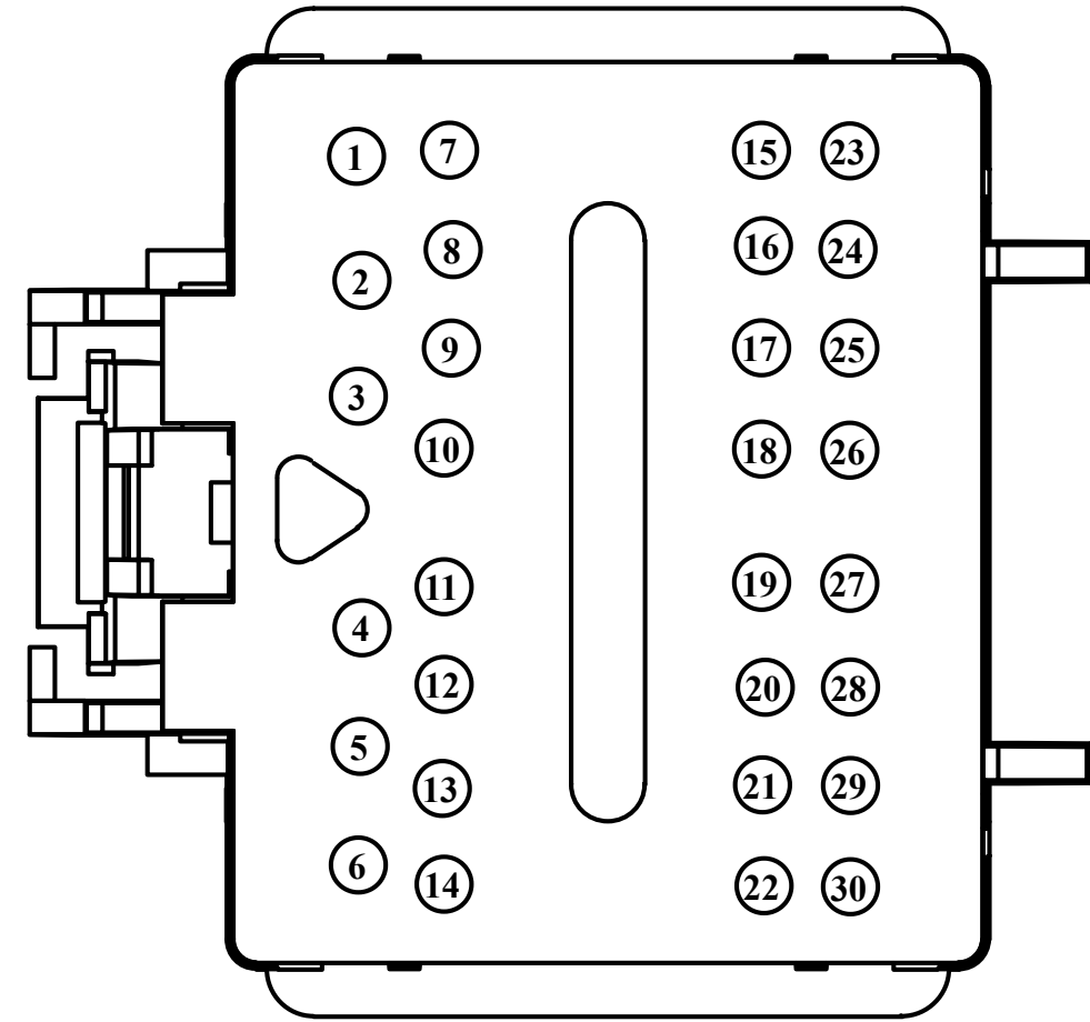
FEMALE Harness 14401
